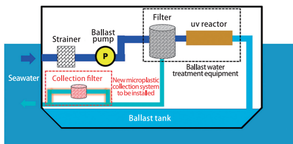
Image of microplastic collection device
